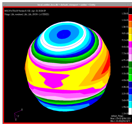
Fatigue Life of Solder Joint
